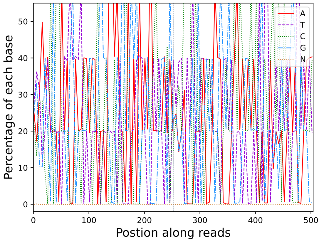
Base percentage along reads (R20205)
